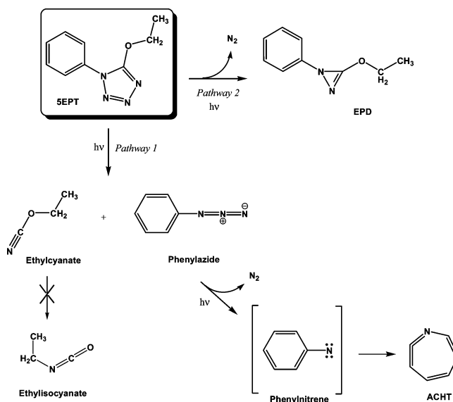
SCHEME 1: Proposed Pathways Resulting from Irradiation of 5-Ethoxy-1-phenyl-1H-tetrazole in an Argon Matrix through the Outer KBr Window of the Cryostat ( \lambda > 235 \text{ nm} )
