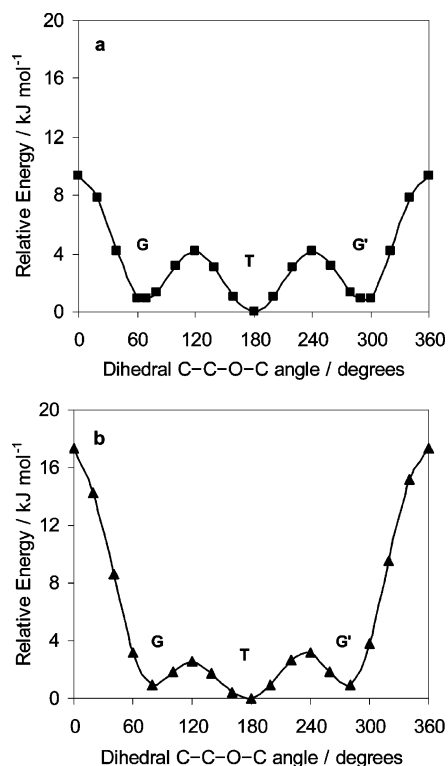
Figure 5. DFT(B3LYP)/6-311++G(d,p) calculated potential energy profiles for internal rotation of the ethoxy group around the C_{(4)}-O_{(1)} bond in ethylcyanate (EC) (a) and 3-ethoxy-1-phenyl-1 H -diazirene (EPD) (b). The energies of the conformers T (the lowest energy structures) are equal to -247.338\ 011 and -533.742\ 444 hartrees for EC and EPD, respectively (without the ZPE contribution) and were chosen as the relative zero levels. Minima denoted G , T , and G' on the curve correspond to the lower energy conformers (Tables S6, S7, and S10–S12, Supporting Information).
